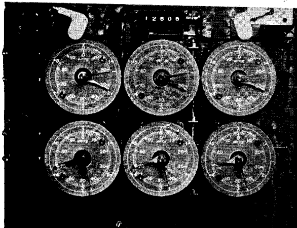
Front View of Walker Propeller Log Without Case
