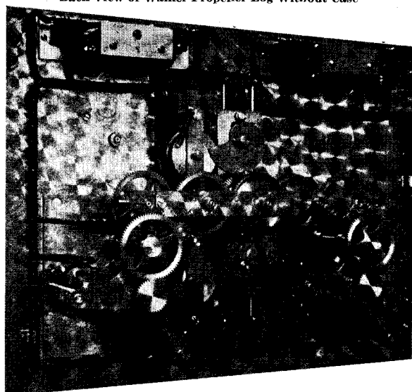
Back View of Walker Propeller Log Without Case
