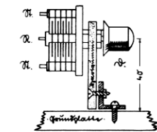
O b e n : Montage des Differentials.
